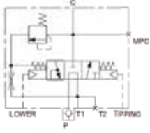
HİDROLİK SEMBOL HYDRAULIC SYMBOL
