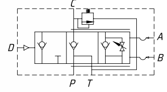
HİDROLİK SEMBOL HYDRAULIC SYMBOL
