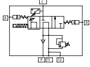
HİDROLİK SEMBOL HYDRAULIC SYMBOL
